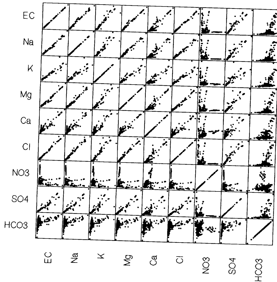
Fig. 38. Correlation of EC, cations and anions in the coastal spring water.
