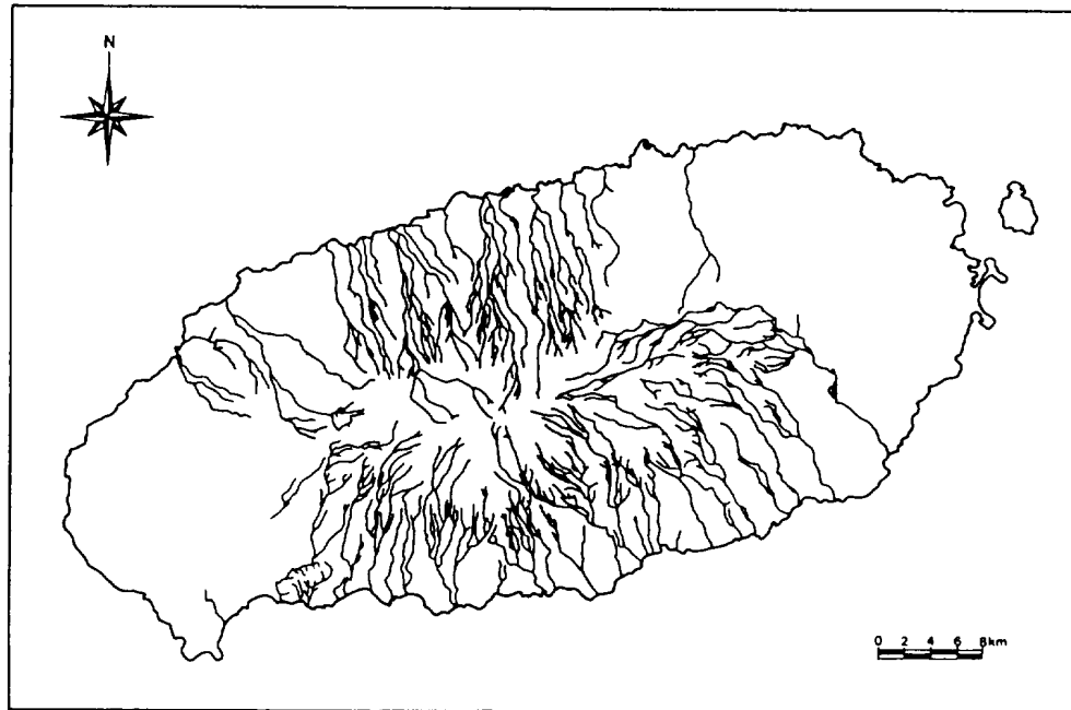
Fig. 5. Waterways of the study area(WRDC, 1993).
