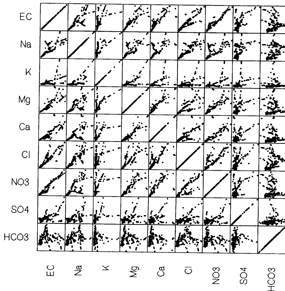
Fig. 37. Correlation of EC, cations and anions in the low mountain spring water.
