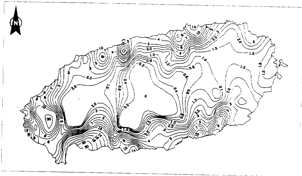
Fig. 48. Iso-concentration line map of nitrate nitrogen( \text{NO}_3^- - \text{N} ) concentration(ppm).
