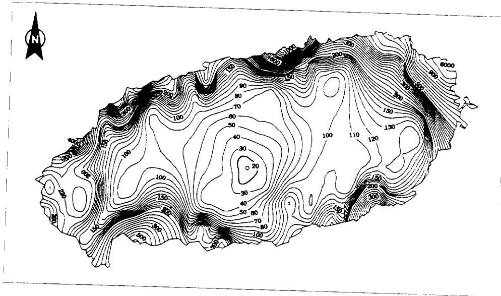
Fig. 40. Iso-concentration line map of electrical conductivity(EC)( \mu\text{S/cm} ).
