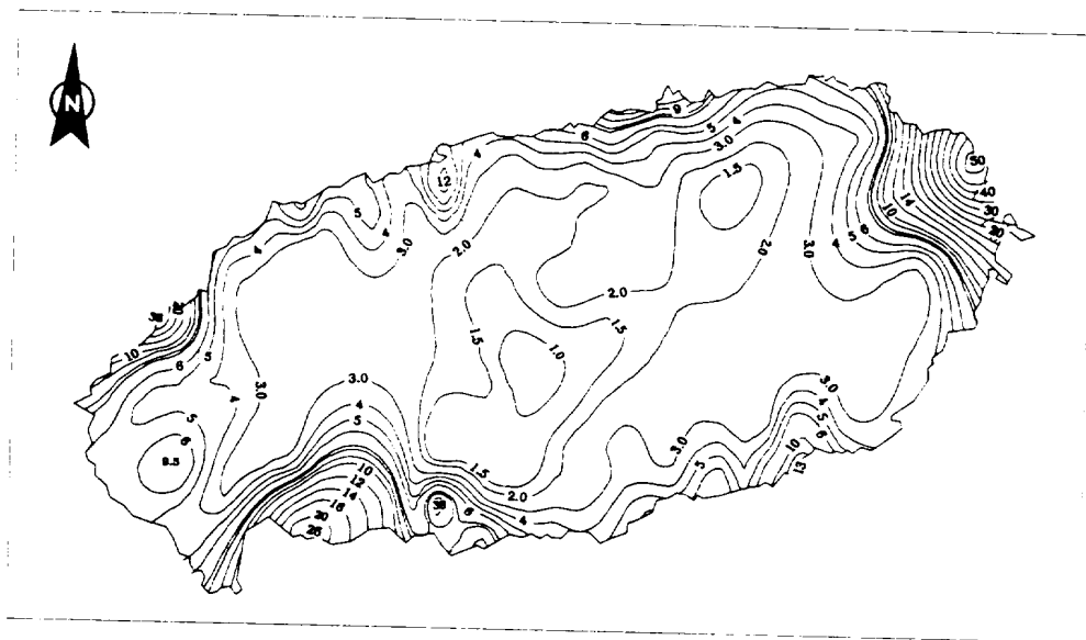
Fig. 44. Iso-concentration line map of calcium( \text{Ca}^{2+} ) concentration(ppm).
