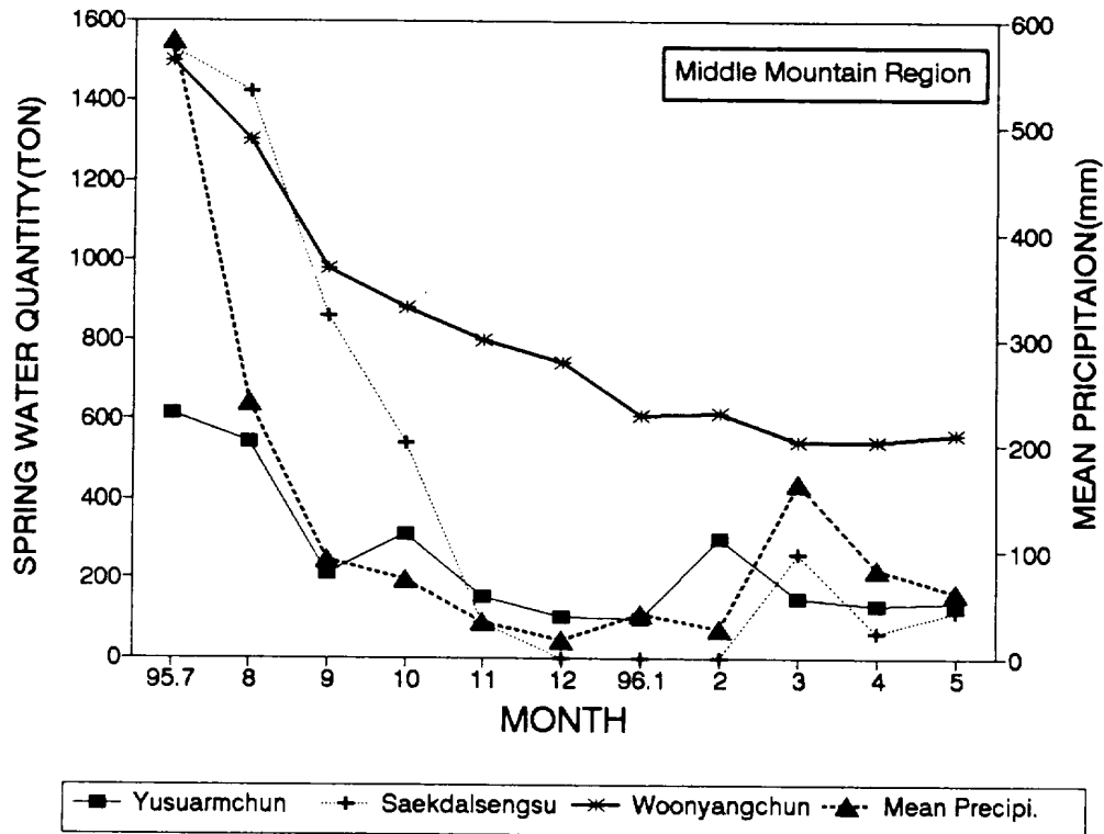
Fig. 8. Monthly variations of spring water quantity and mean precipitation in the middle mountain region.
