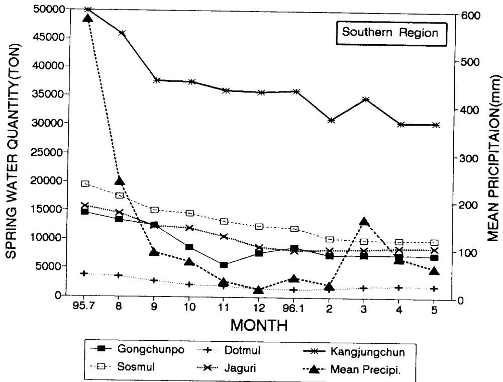
Fig. 11. Monthly variations of spring water quantity and mean precipitation in the southern region.
