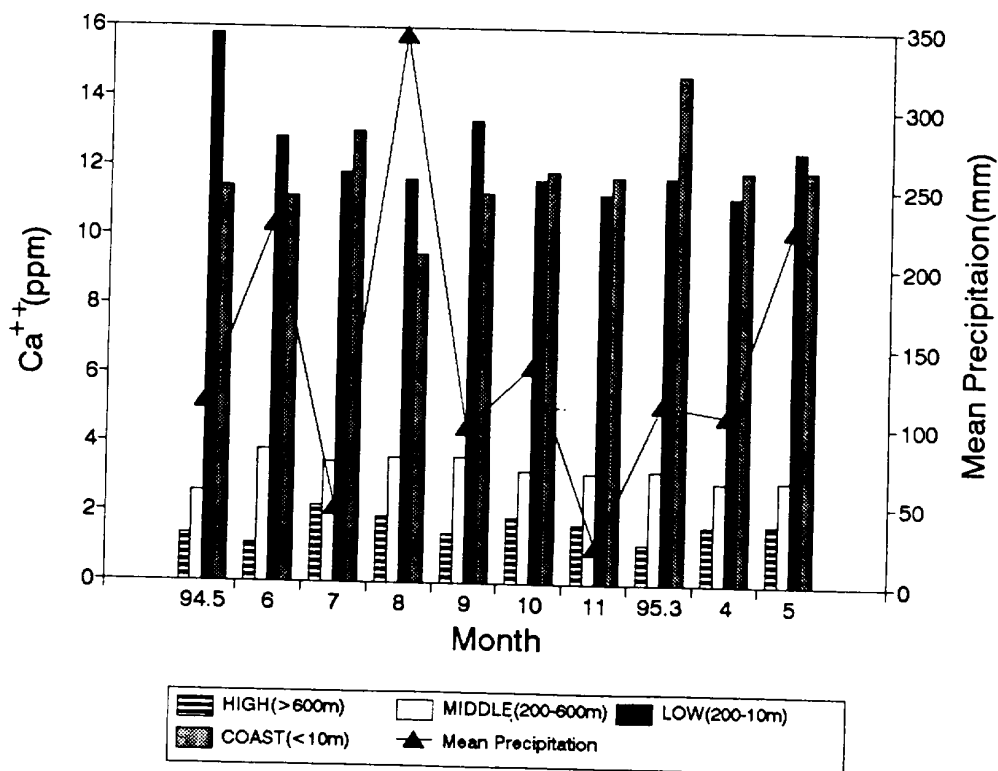
Fig. 24. Monthly variations of calcium concentration and precipitation.
